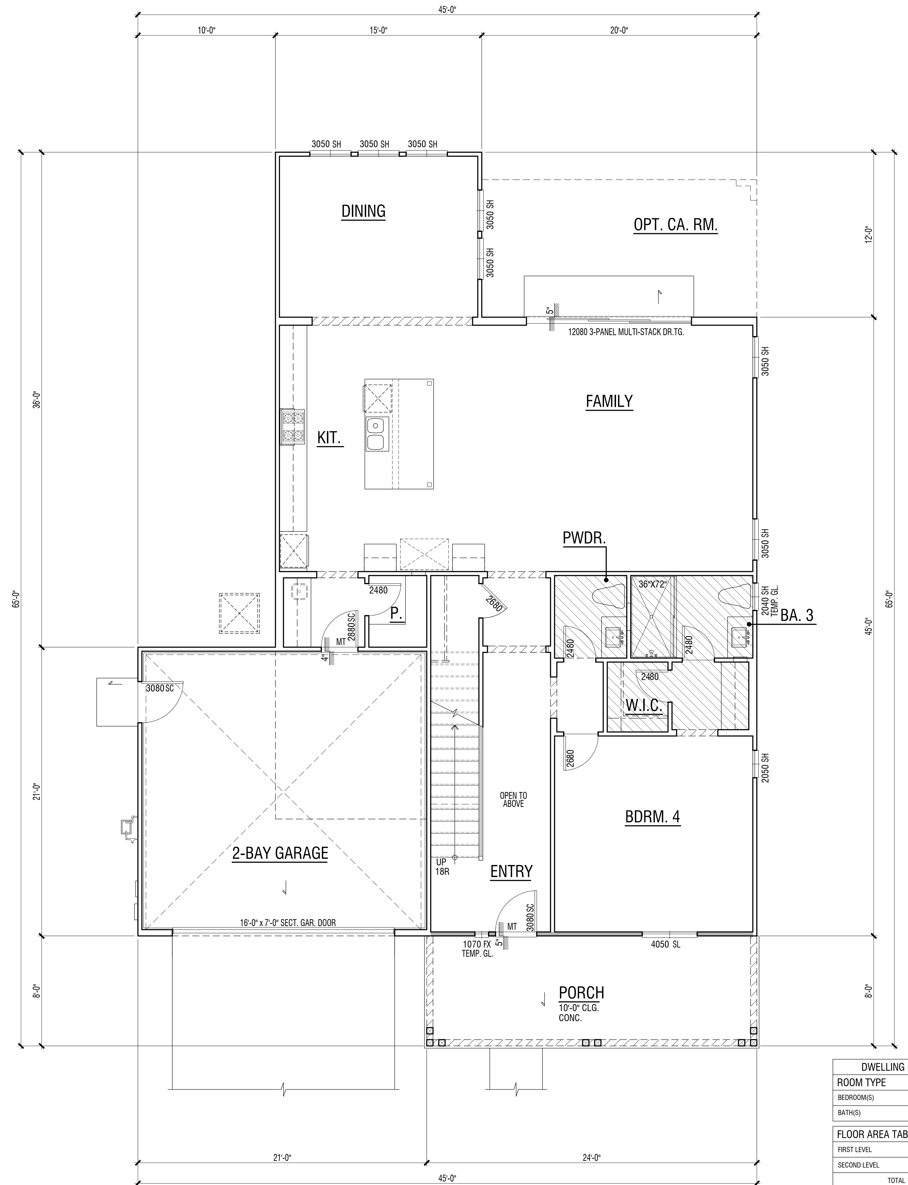
PLAN 2D | 'American Cottage' Floor Plan
