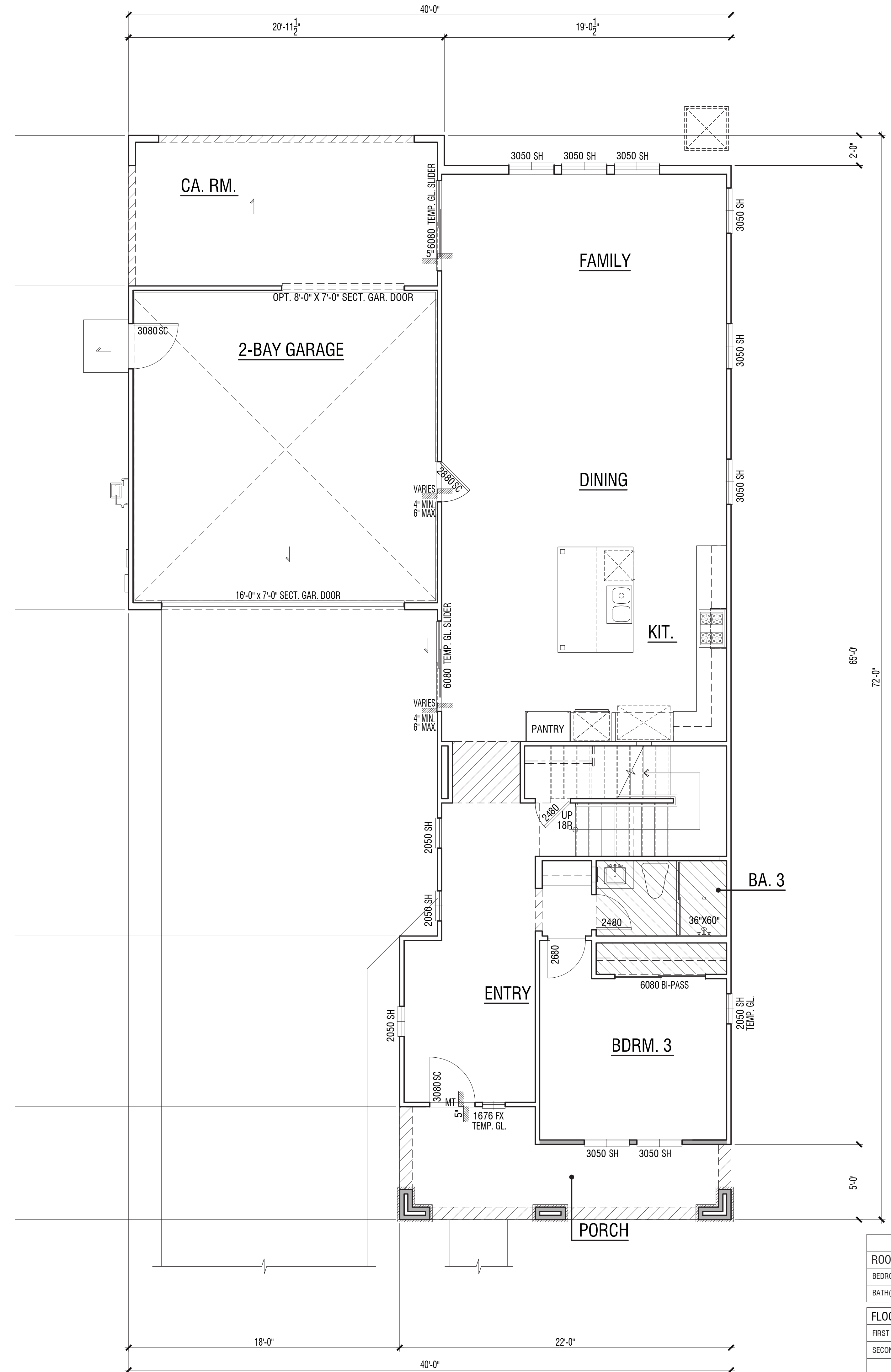
PLAN 1C | 'California Craftsman' Floor Plan
