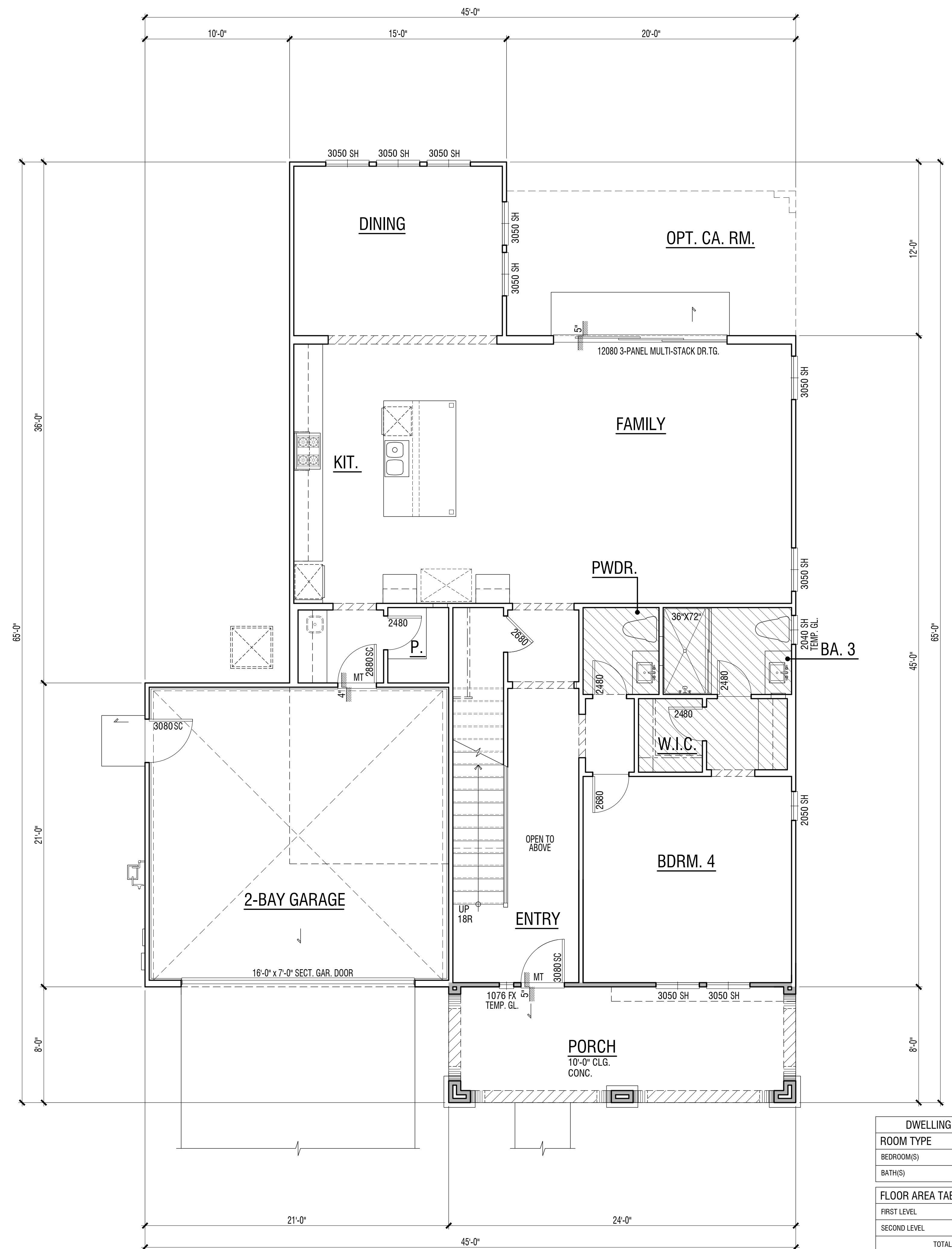
PLAN 2B | 'California Bungalow' Floor Plan
