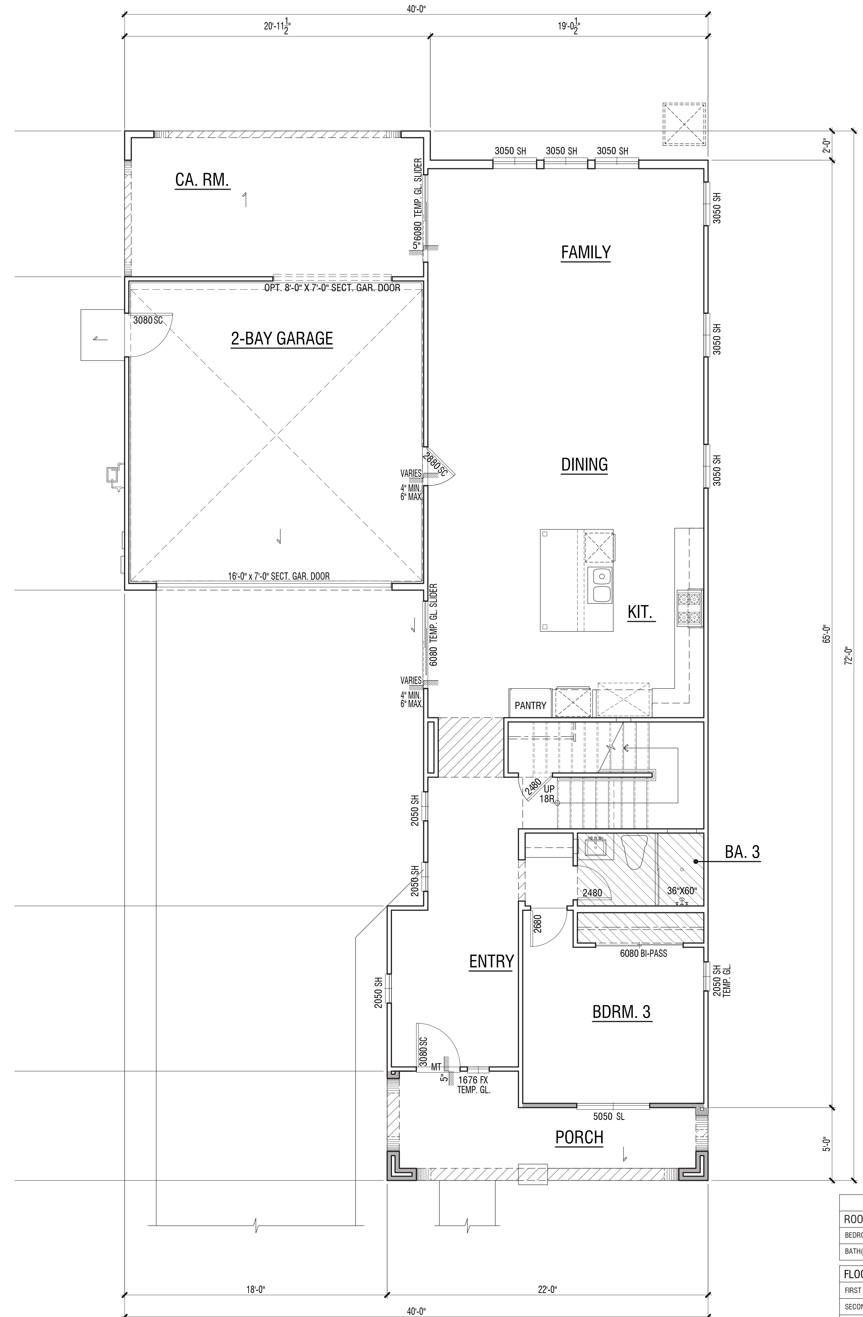
PLAN 1B | 'California Bungalow' Floor Plan
